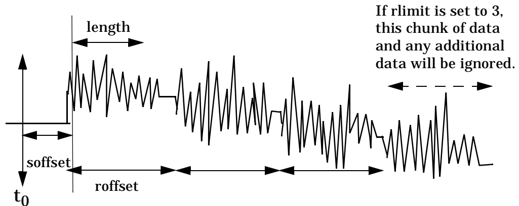
Figure 0-2 Sample Trace Data - Not Constant Envelope
