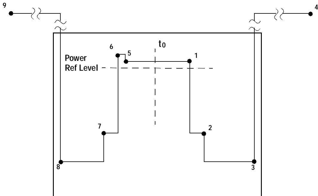
Figure 0-5 Custom Upper Limit Mask Example
