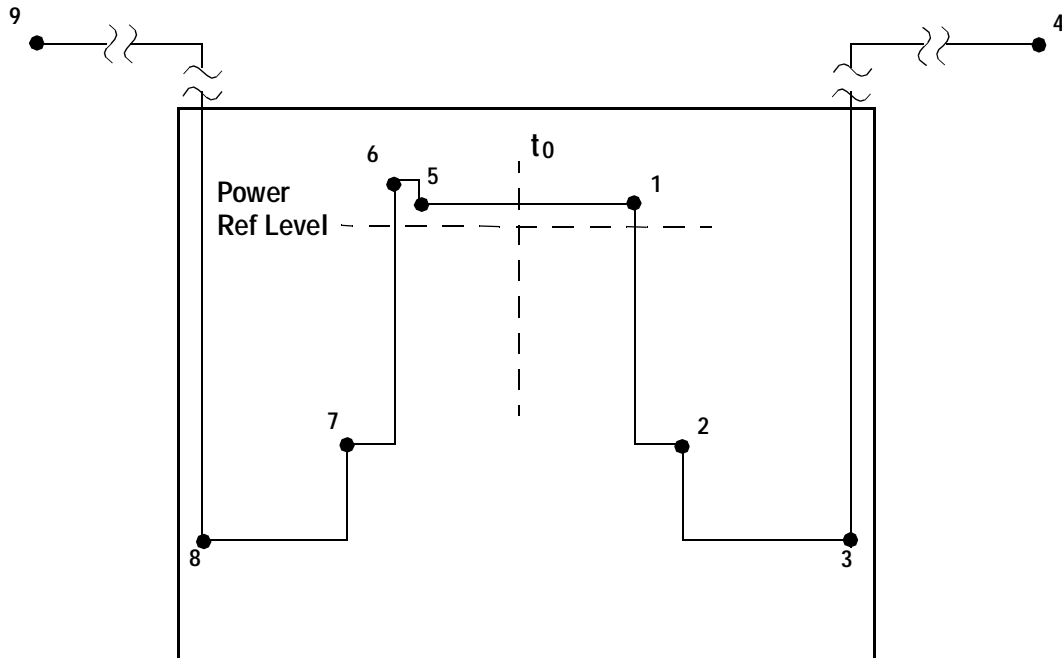
Figure 0-4 Custom Upper Limit Mask Example
